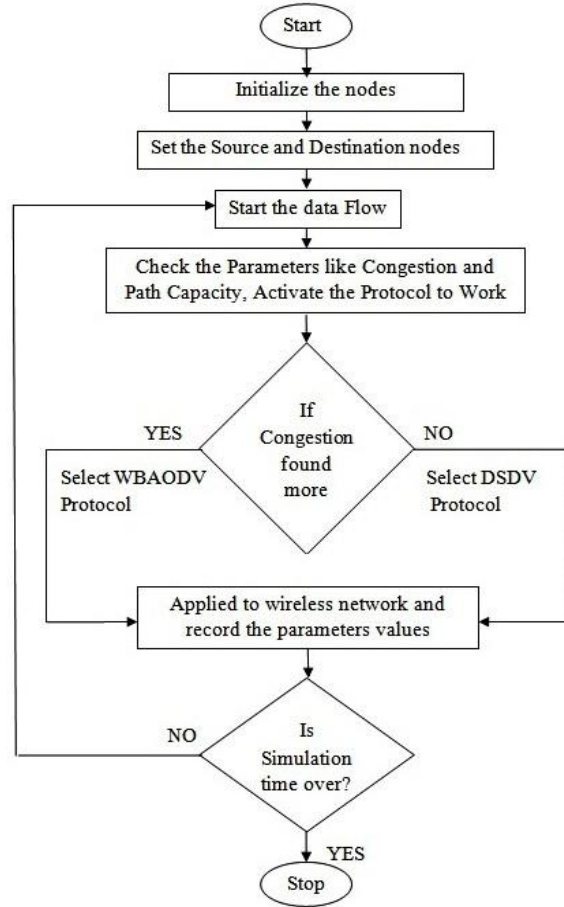
Figure 1. Hybrid routing protocol mechanism flowchart
