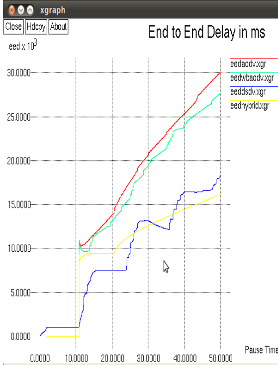
Figure 2: Comparative analysis of End to End Delay
