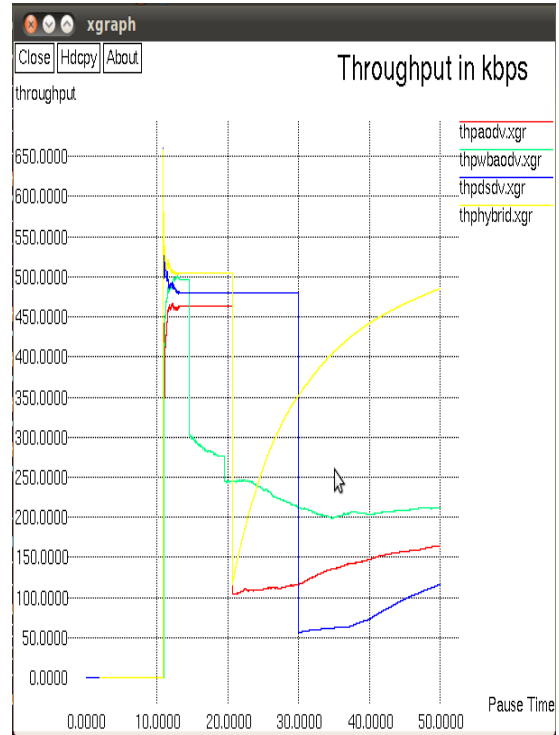
Figure 3: Comparative analysis of Throughput
